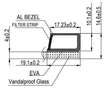
Section A-A Detail 5:1
