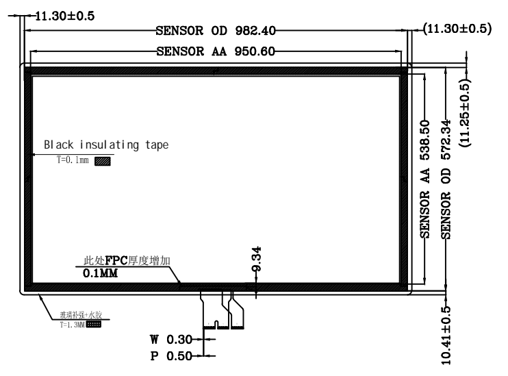
Back view
