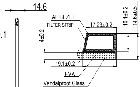
Section A-A Detail 5:1
