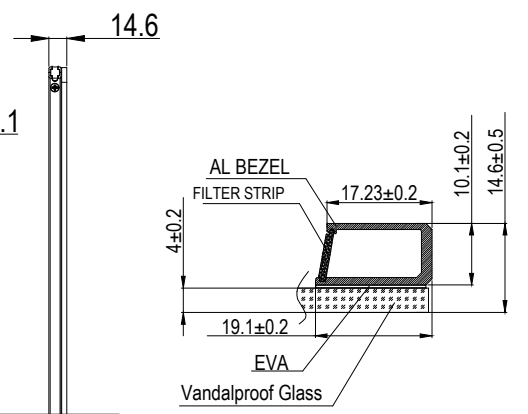
Section A-A Detail 5:1
