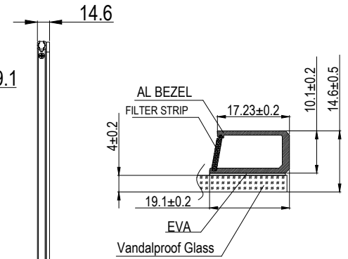
Section A-A Detail 5:1
