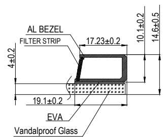
Section A-A Detail 5:1
